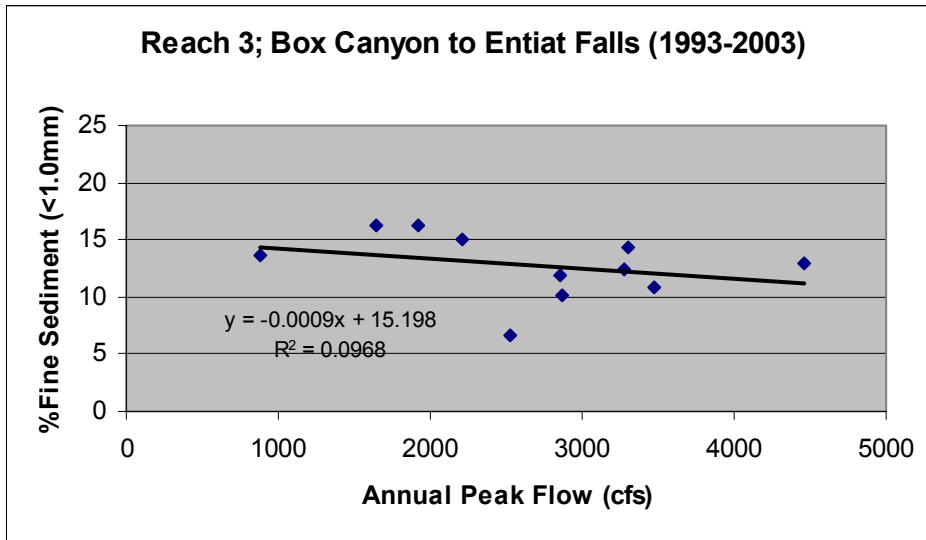
Figure 5. Percent fine sediment in Reach 3 vs annual peak flow.
