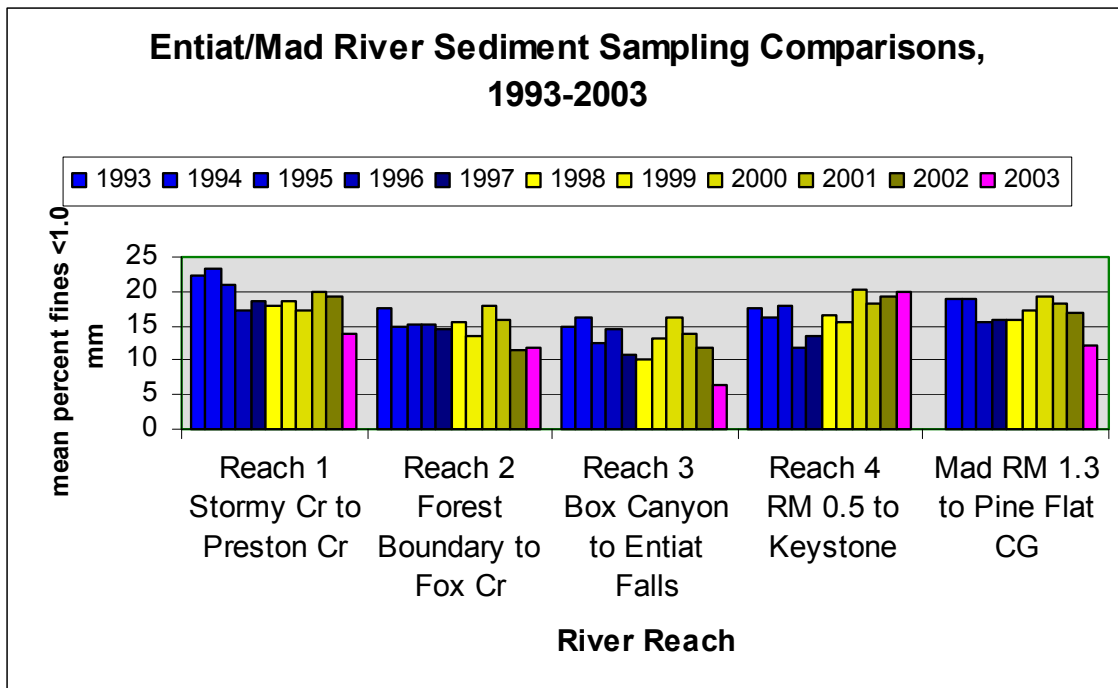
Figure1. Entiat and Mad Rivers Fine Sediment Sampling Comparisons, 1993-2003.
