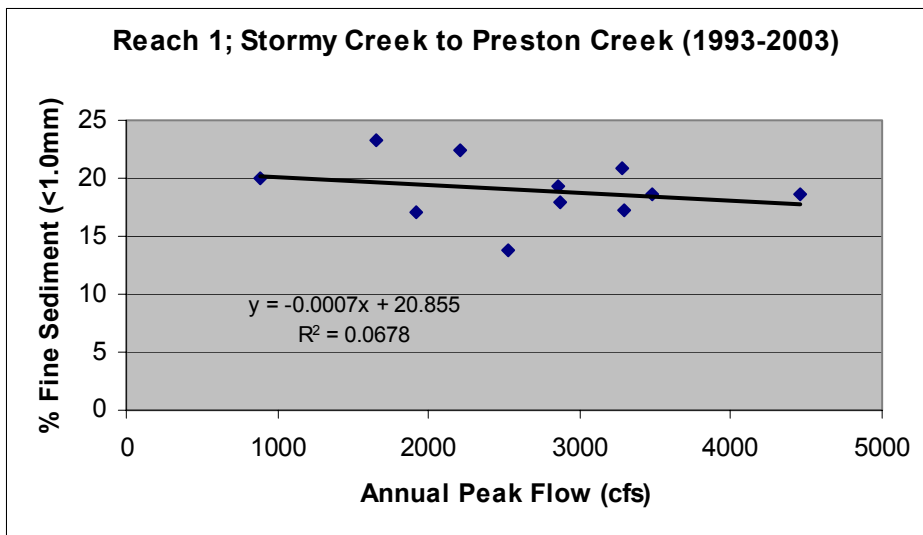
Figure 3. Percent fine sediment in Reach 1 vs annual peak flow.
