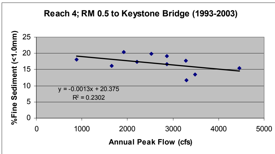
Figure 6. Percent fine sediment in Reach 4 vs annual peak flow.
