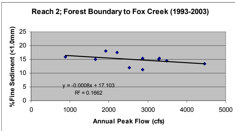
Figure 4. Percent fine sediment in Reach 2 vs annual peak flow.
