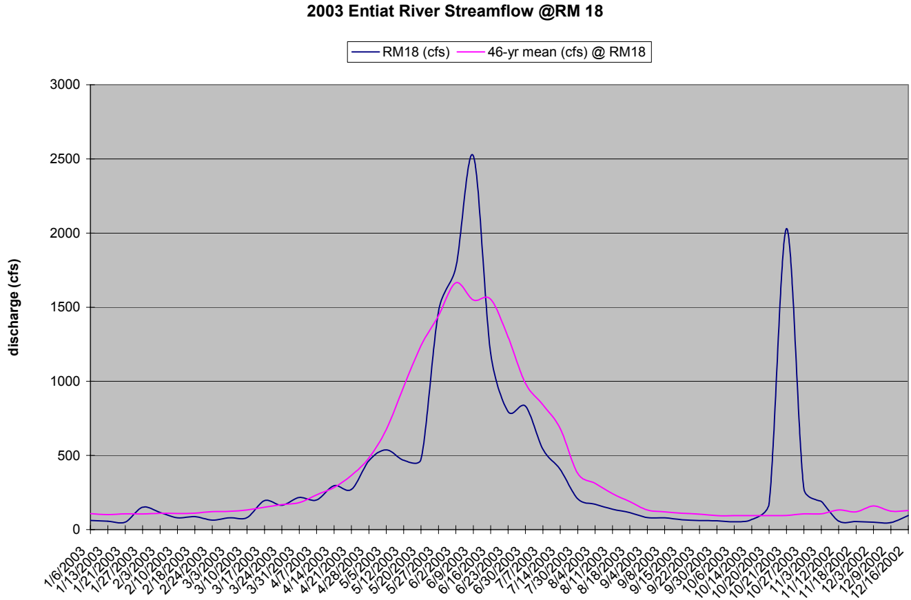
Figure 2. 2003 Entiat River streamflow versus the 46-year mean.
